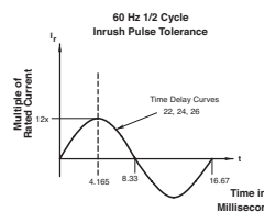
Pulse Tolerance Curve
