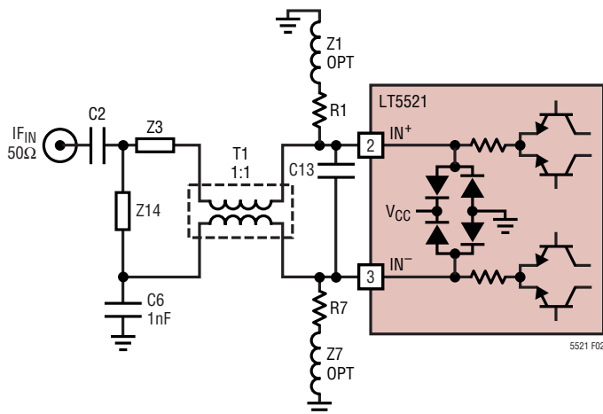
Figure 2. Signal Input with External Matching
