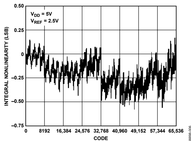
Figure 12. Integral Nonlinearity vs. Code
