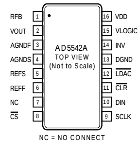
Figure 10. AD5542A 16-Lead TSSOP Pin Configuration
