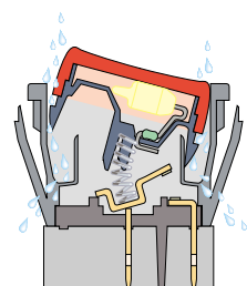
Water-thru Integral splashproof system (pat app.)
