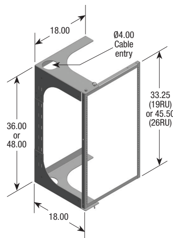
XWR Swing-out Style Wall Mount Rack
