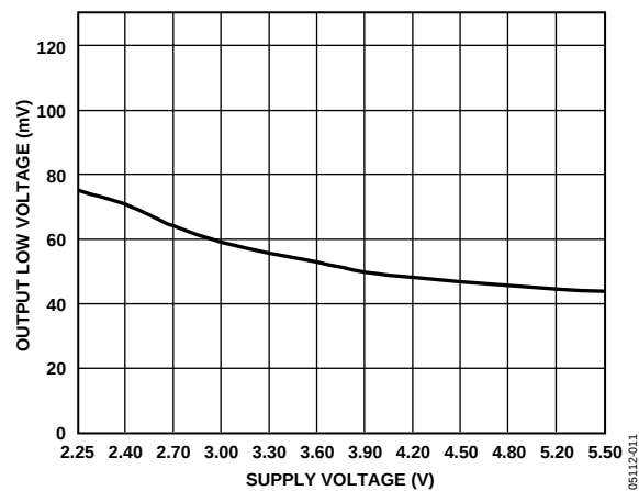
Figure 13. Output Low Voltage vs. Supply Voltage ( I_{SINK} = 500 mA )
