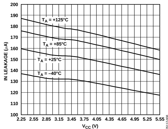
Figure 9. Input Leakage vs. Supply Voltage ( V_{IN} = 22 V )
