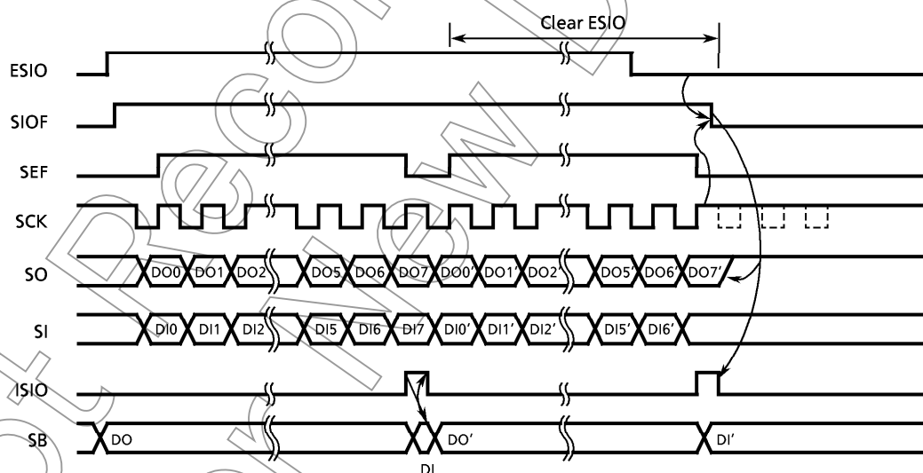
Figure3-30. 8-bit Transmit/Receive Mode
