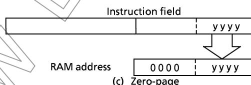
Figure 2-5. Addressing mode
