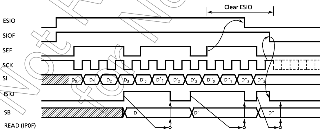
Figure3-29. 4-bit Receive Mode
