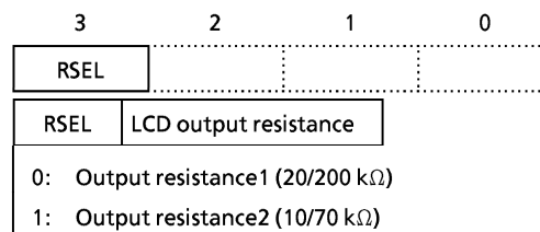
Figure 3-32. Command Register
