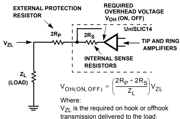
FIGURE 16. OVERHEAD VOLTAGE OF THE TIP AND RING AMPLIFIERS
