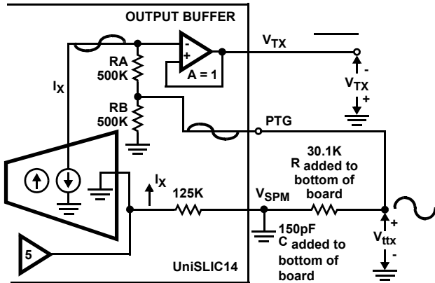
FIGURE 23. PULSE METERING WITH TRANSYBRID BALANCE
