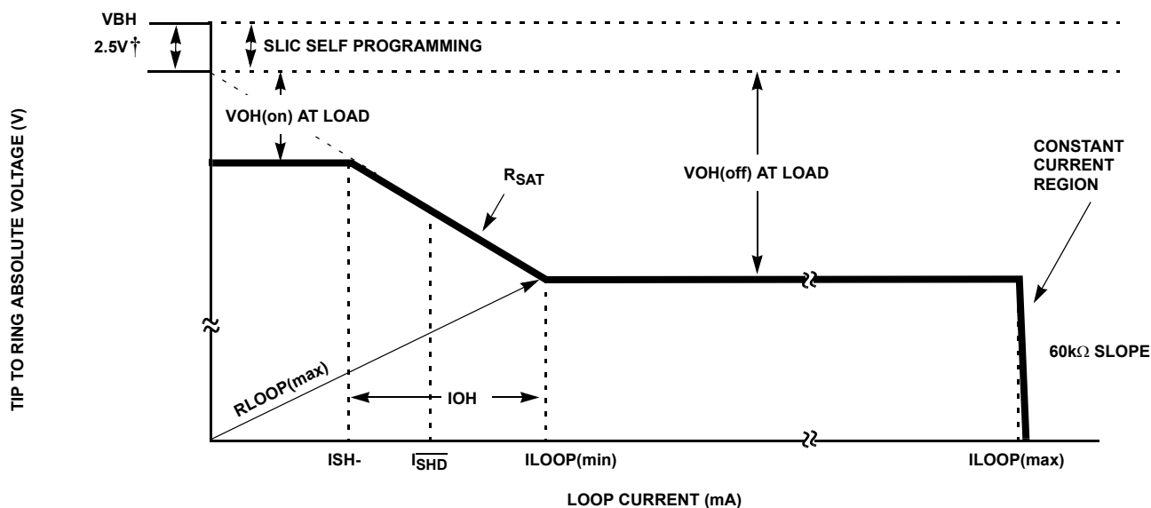
FIGURE 15. UniSLIC14 DC FEED CURVE
