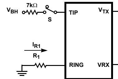
FIGURE 11. TIPX VOLTAGE
