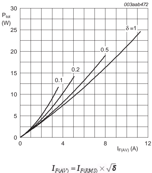
Fig 2. Forward power dissipation as a function of average forward current; square waveform; maximum values
