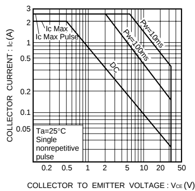
Fig.10 Safe operating area (2SD1862)
