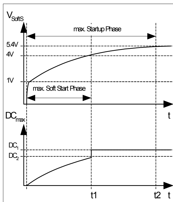
Figure 5 Startup Phase
