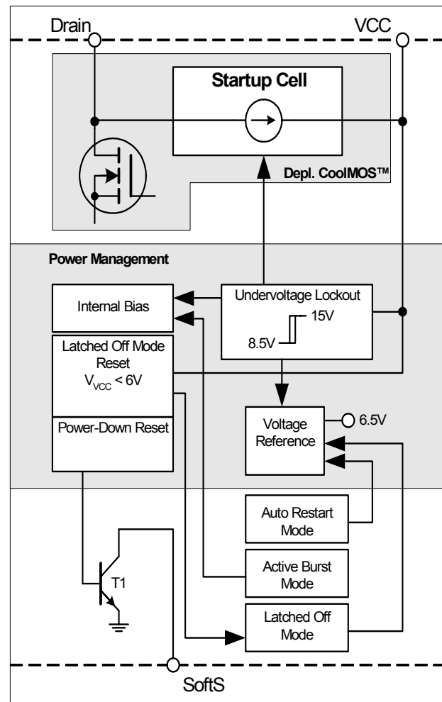
Figure 3 Power Management
