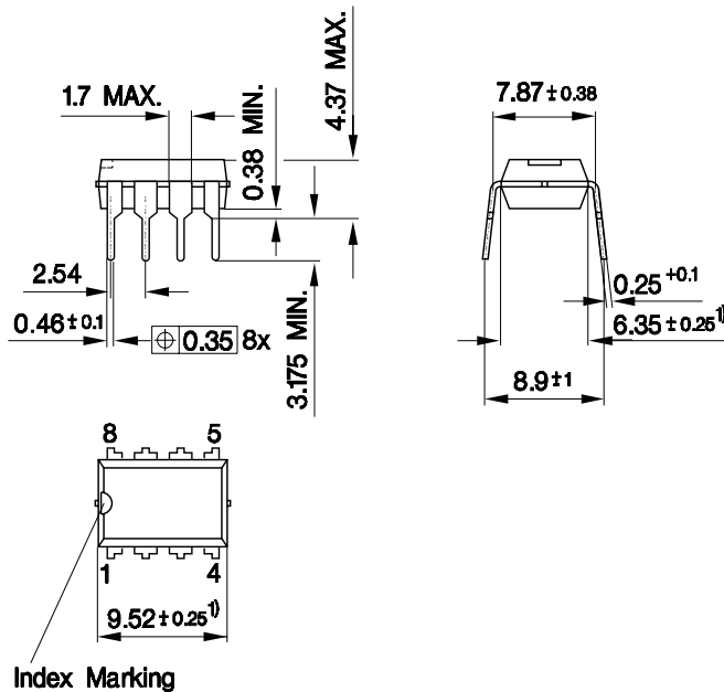
Figure 24 PG-DIP-8-6 ( Pb-free lead plating Plastic Dual-in-Line Outline )
