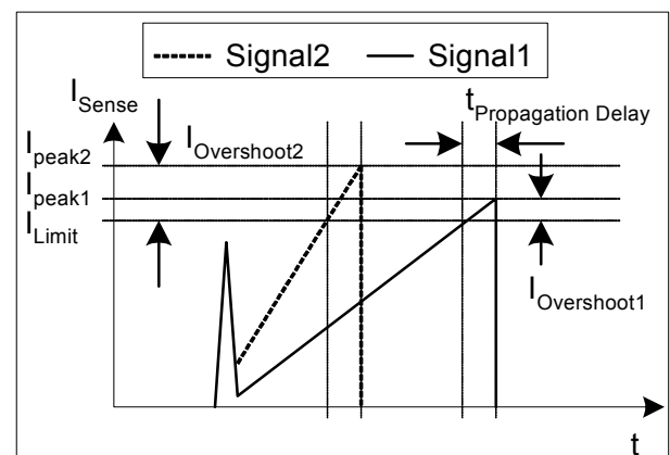
Figure 11 Current Limiting
