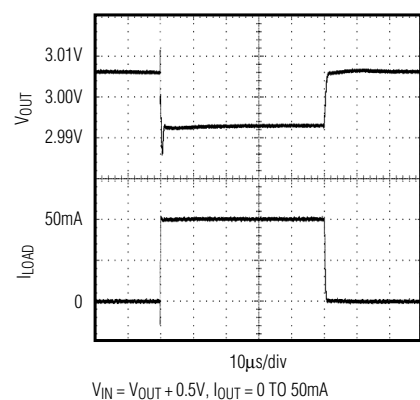
LOAD-TRANSIENT RESPONSE
