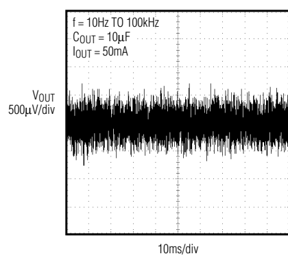
OUTPUT NOISE
