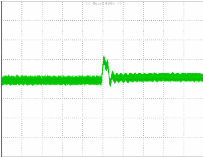
Figure 8: Output voltage response to step-change in load current (75%-50% of I_o , max; di/dt = 0.1A/\mu S ). Load cap: 10uF Low ESR capacitor and 1uF ceramic capacitor. Top Trace: Vout (50mV/div), Scope measurement should be made using a BNC cable (length shorter than 20 inches). Position the load between 51 mm to 76 mm (2 inches to 3 inches) from the module.
