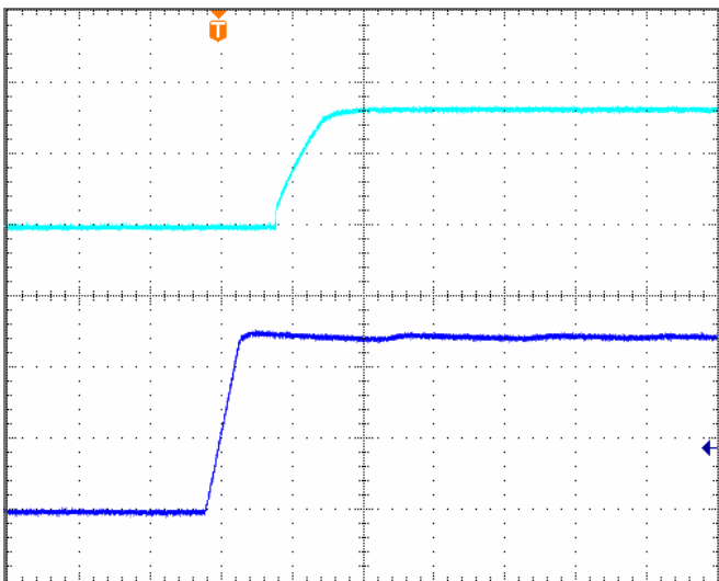
Figure 7: Turn-on transient at zero load current (10ms/div). CH2 Vout: 2V/div; CH1:Vin: 20V/div
