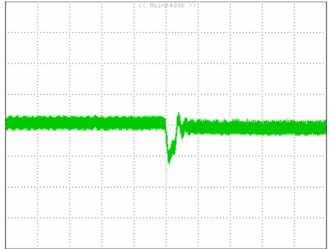
Figure 9: Output voltage response to step-change in load current (50%-75% of I_o , max; di/dt = 0.1A/\mu S ). Load cap: 10uF Low ESR capacitor and 1uF ceramic capacitor. Top Trace: Vout (50mV/div), Scope measurement should be made using a BNC cable (length shorter than 20 inches). Position the load between 51 mm to 76 mm (2 inches to 3 inches) from the module.
