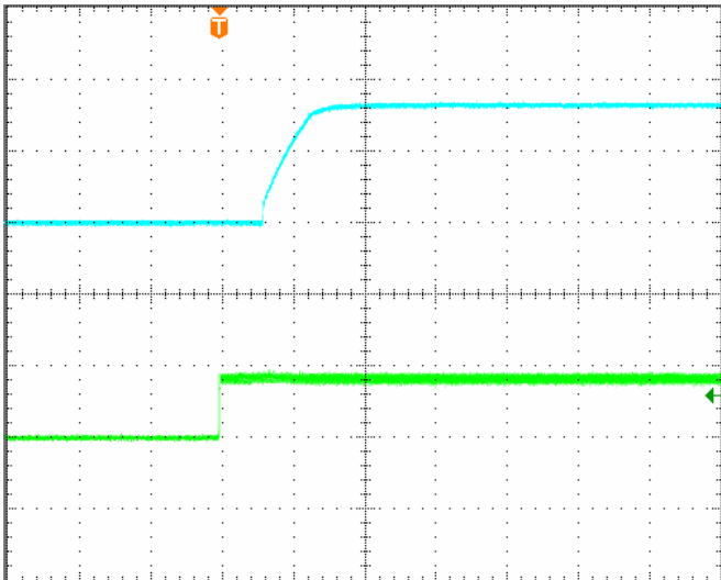
Figure 5: Turn-on transient at minimum load current (10ms/div). CH2: Vout: 2V/div; CH4: ON/OFF input: 5V/div
