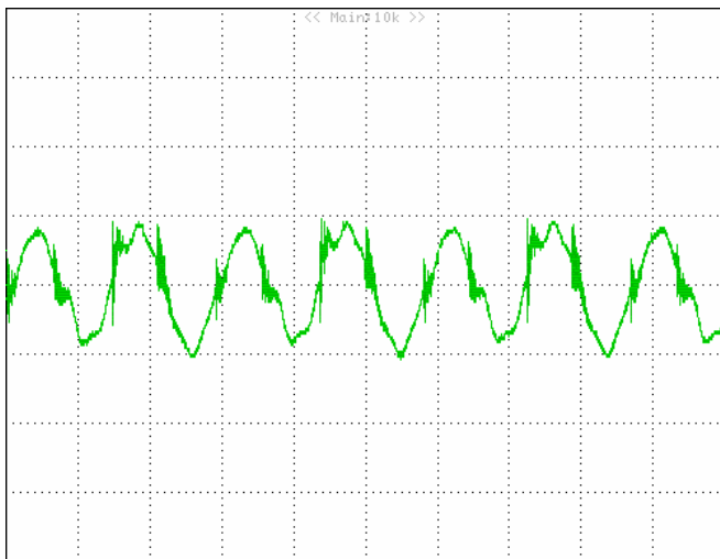
Figure 14: Output voltage ripple at nominal input voltage and rated load current (10mV/div). Load capacitance: 1\mu\text{F} ceramic capacitor and 10\mu\text{F} Flow ESR capacitor. Bandwidth: 20 MHz. Scope measurement should be made using a BNC cable (length shorter than 20 inches). Position the load between 51 mm to 76 mm (2 inches to 3 inches) from the module.
