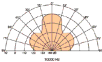
radiation pattern 10000 Hz
