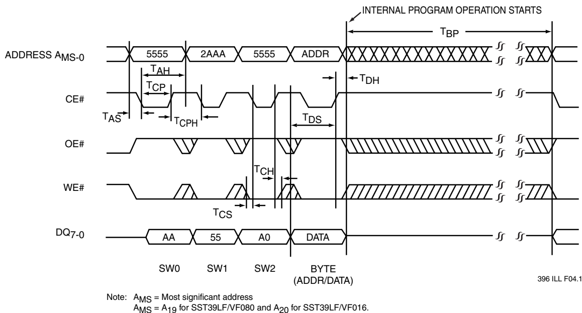
FIGURE 5: CE# CONTROLLED PROGRAM CYCLE TIMING DIAGRAM
