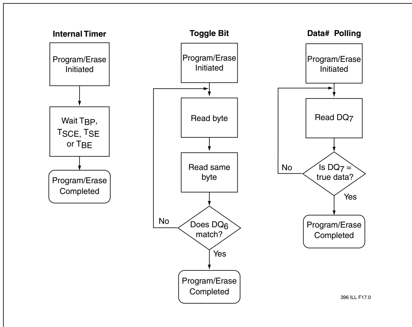
FIGURE 17: WAIT OPTIONS
