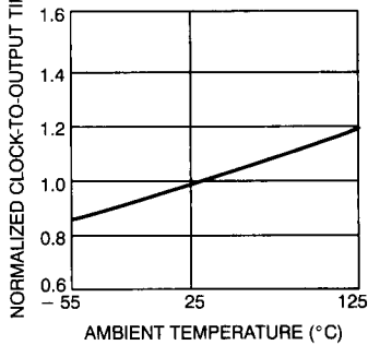
CLOCK TO OUTPUT TIME vs. TEMPERATURE
