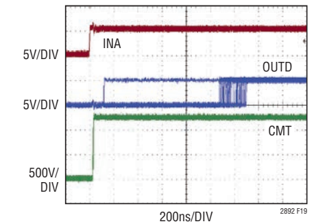
Figure 19. Data Refresh Recovery for 200kV/ \mu s Transient
