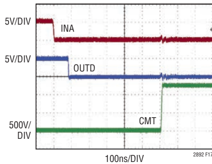
Figure 17. Static Operation with 200kV/ \mu s Transients
