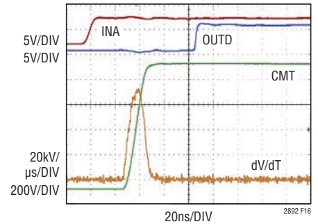
Figure 16. Transient dV/dT, 70kV/ \mu s
