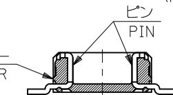
SECT.W-W(LOCK PART)
