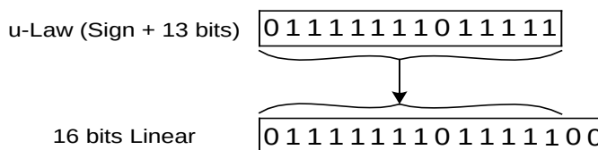
Figure 25: Mapping of μ-law Code to 16-bit Code
