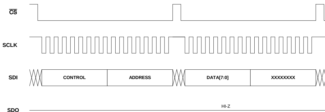
Figure 18: SPI Write Transaction – 16-bit Mode
