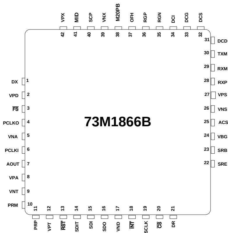
Figure 6: 73M1866B 42-Pin Pinout
