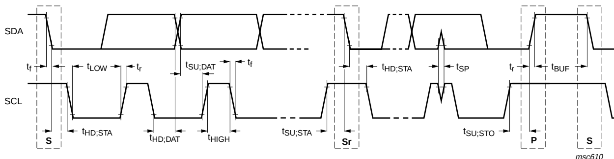
Fig 4. I 2 C-bus timing
