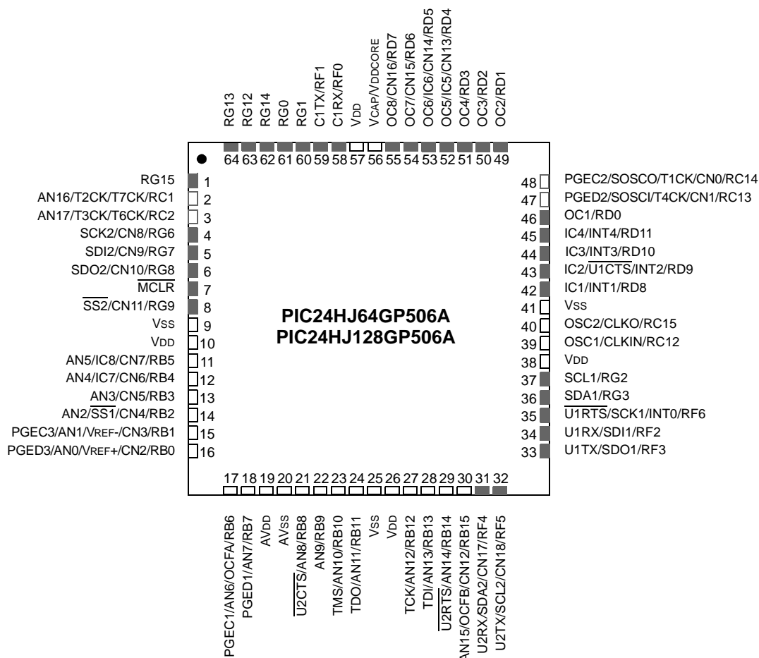
64-Pin QFN (1)
