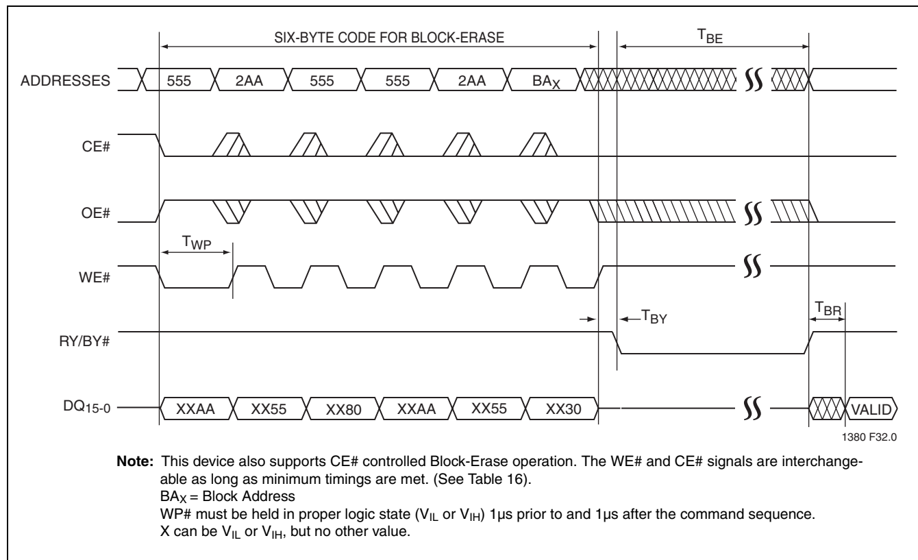
FIGURE 12: WE# Controlled Block-Erase Timing Diagram
