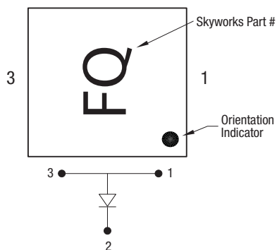
Figure 8. Typical Case Markings (Top View)
