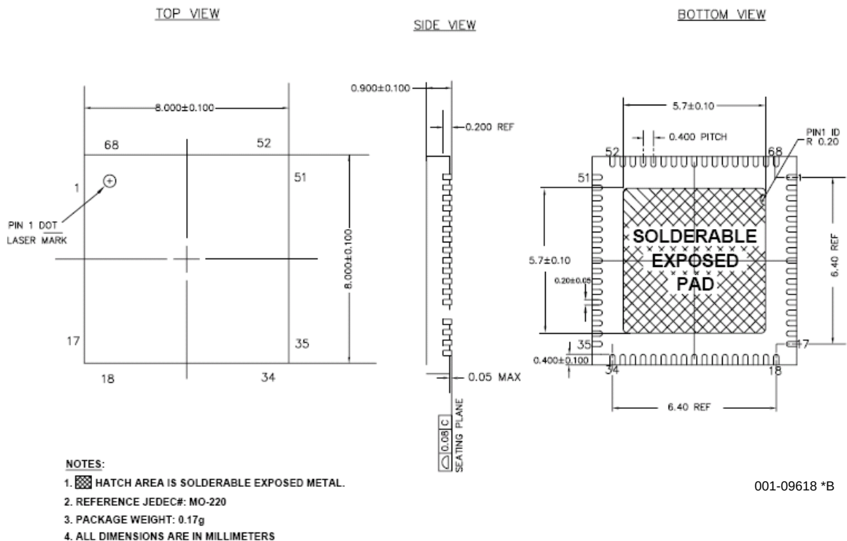
Figure 11-4. 68-Pin Sawn QFN (8X8 mm X 0.90 mm)
