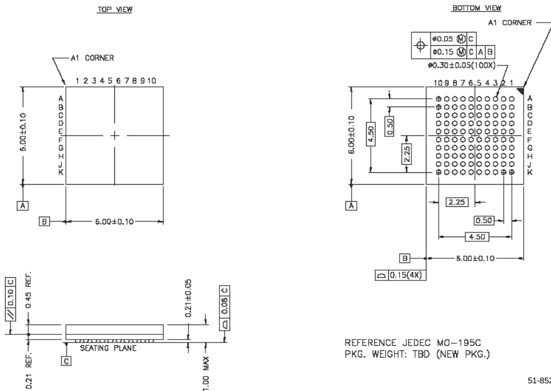
Figure 11-5. 100-Ball (6x6 mm) VFBGA
