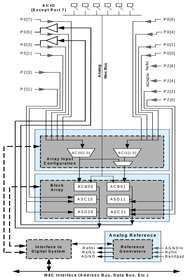
Figure 3-2. Analog System Block Diagram
