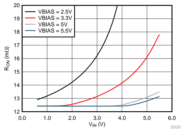
Figure 35. R_{ON} vs V_{IN}
