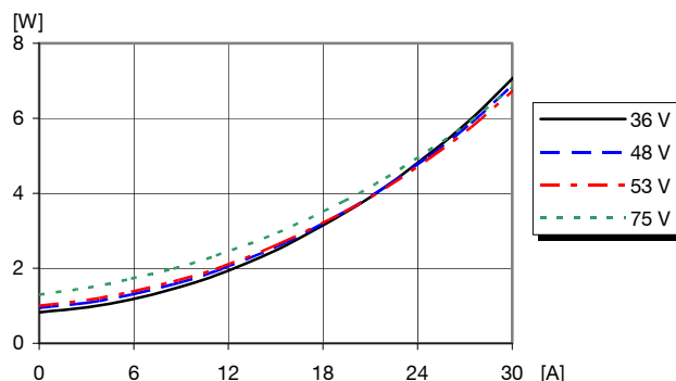
Dissipated power vs. load current and input voltage at T_{ref} = +25^{\circ}\text{C}
