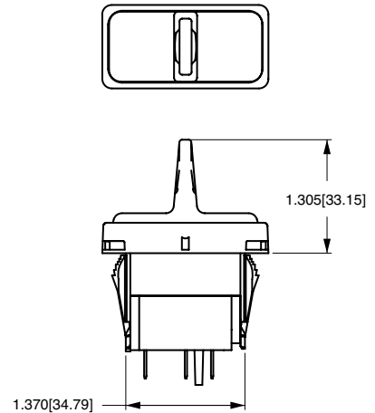
8 TERMINAL BASE W/O BARRIERS
