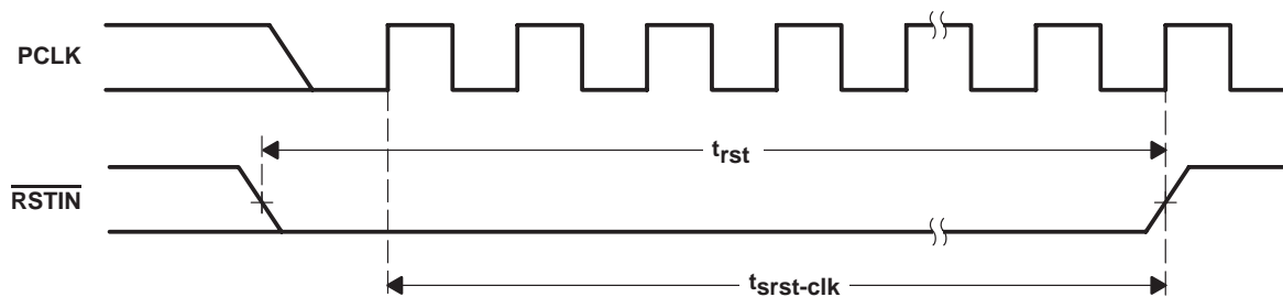
Figure 21. \overline{RSTIN} Timing Waveforms
