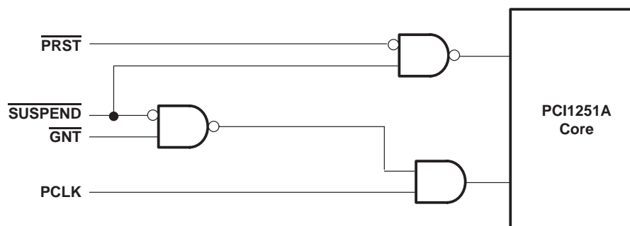
Figure 14. \overline{\text{SUSPEND}} Functional Implementation
