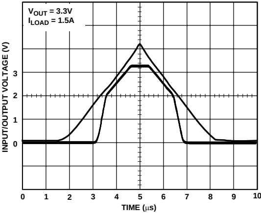
Figure 11. Power-Up/Power-Down
