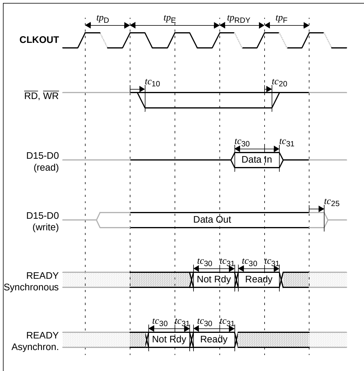
Figure 23 READY Timing
