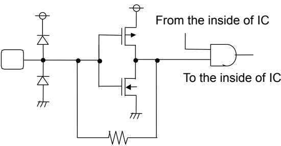
Fig.113 BU3071HFV
