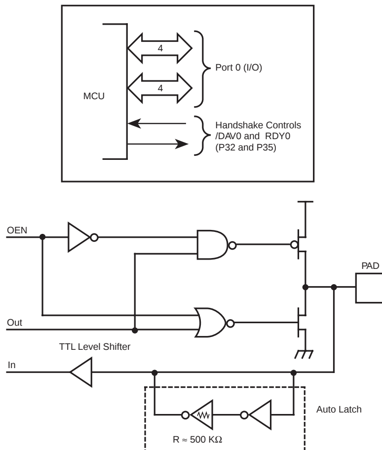
Figure 10. Port 0 Configuration
