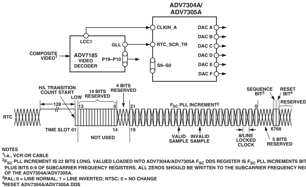
Figure 29. RTC Timing and Connections
