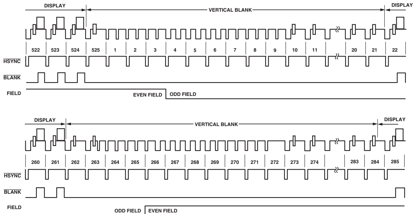
Figure 98. SD Slave Mode 1, NTSC
