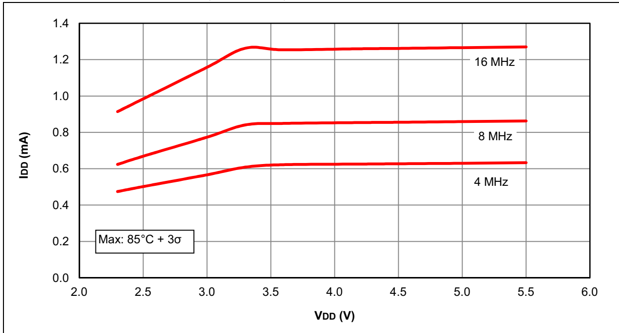
FIGURE 28-20: I DD MAXIMUM, HFINTOSC, PIC12F1501 ONLY
