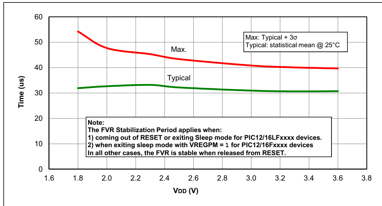
FIGURE 28-52: FVR STABILIZATION PERIOD
