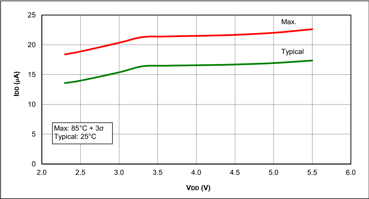
FIGURE 28-14: I_{DD} , LFINTOSC, F_{osc} = 31\text{ kHz} , PIC12F1501 ONLY
