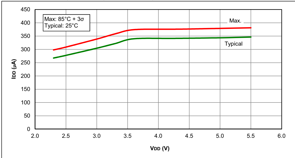
FIGURE 28-16: I_{DD} , MFINTOSC, F_{osc} = 500 kHz, PIC12F1501 ONLY
