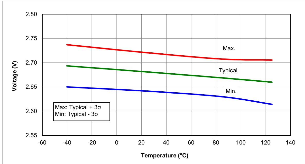
FIGURE 28-47: BROWN-OUT RESET VOLTAGE, BORV = 0
