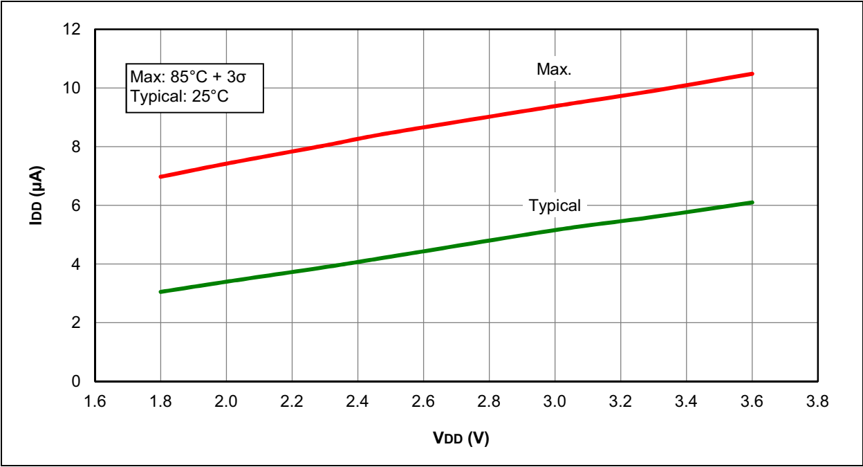
FIGURE 28-13: I_{DD} , LFINTOSC, F_{osc} = 31\text{ kHz} , PIC12LF1501 ONLY
