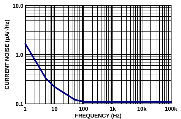
FIGURE 12. ISL28276, ISL28476 CURRENT NOISE vs FREQUENCY
