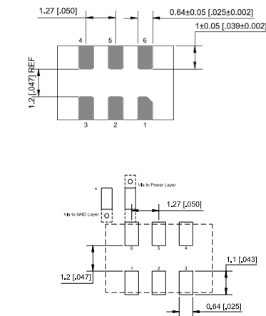
Recommended Land Pattern for LVPECL, LVDS, HCSL
