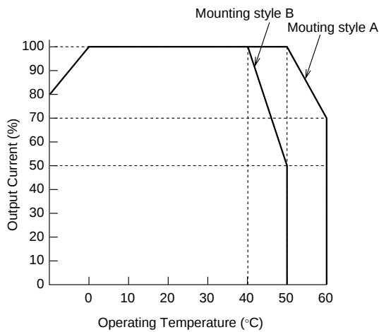
B Mounting
