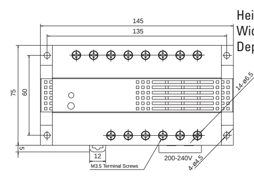
PS5R-E (100W)
