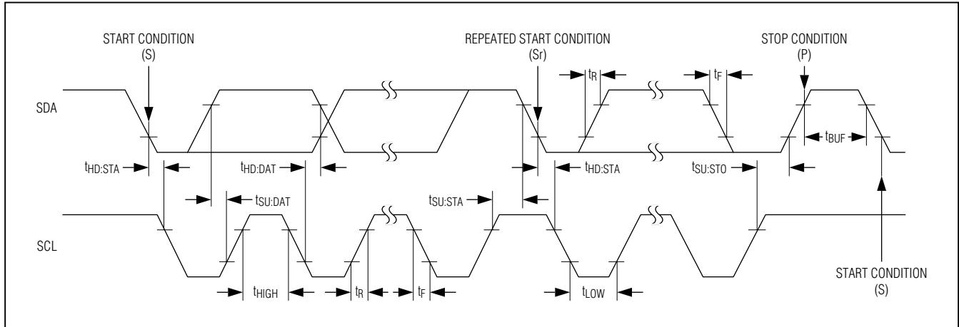
Figure 1. I²C Timing Diagram
