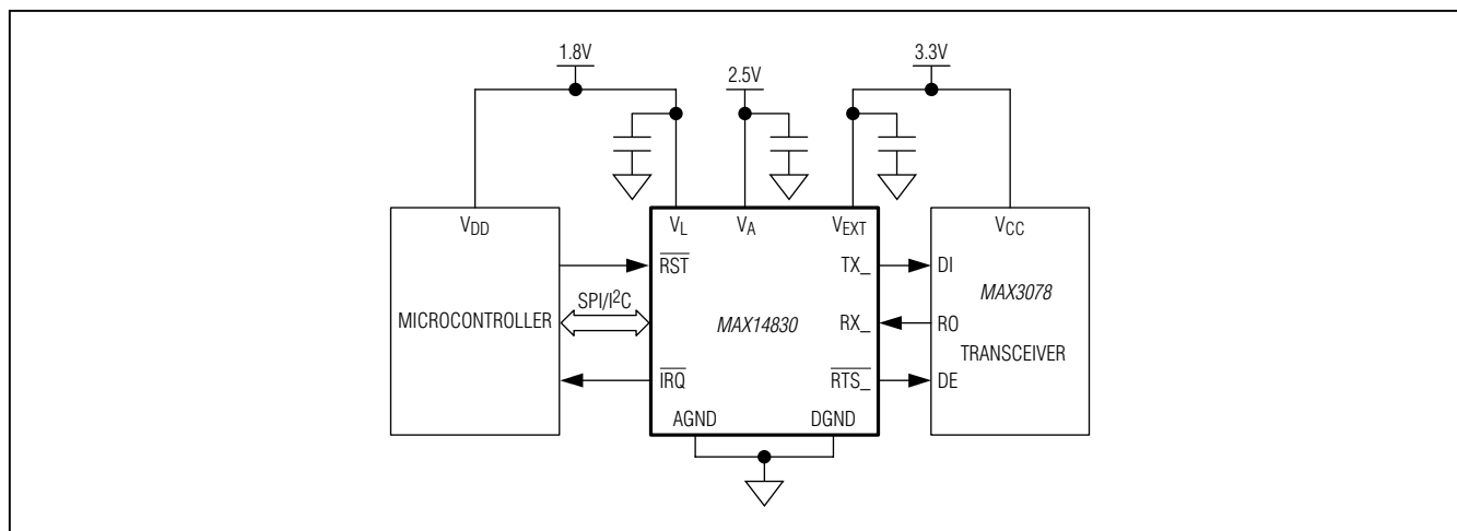
Figure 28. Logic-Level Translation
