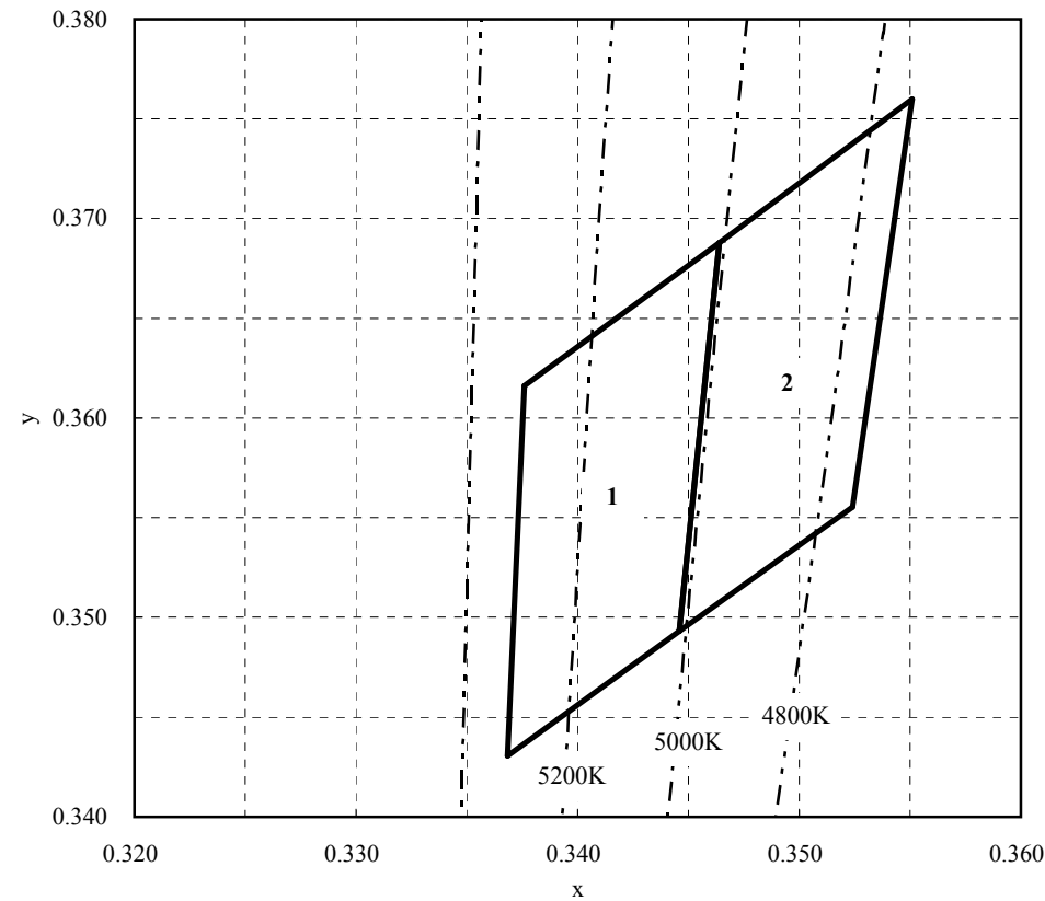
Chromaticity Diagram
