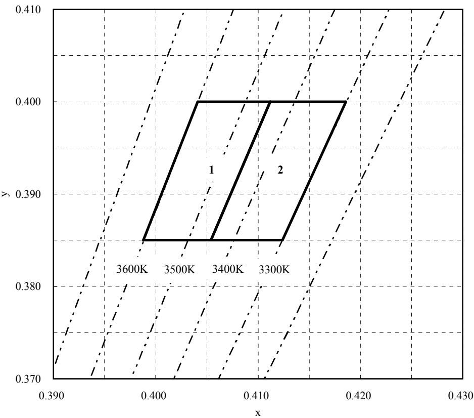
Chromaticity Diagram
