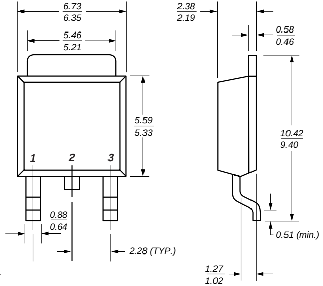
TO-252 (DPAK)
