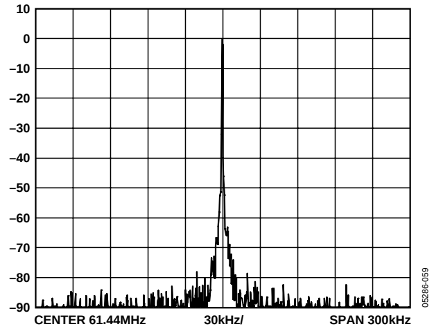
Figure 15. Phase Noise, LVPECL, DIV 4, FVCXO = 245.76 MHz, FOUT = 61.44 MHz, FPDF = 1.2288 MHz, R = 25, N = 200
