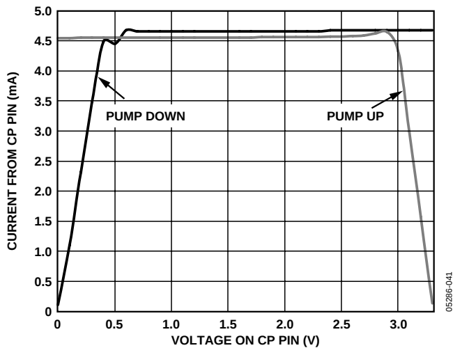
Figure 14. Charge Pump Output Characteristics @ V_{CP5} = 3.3\text{ V}
