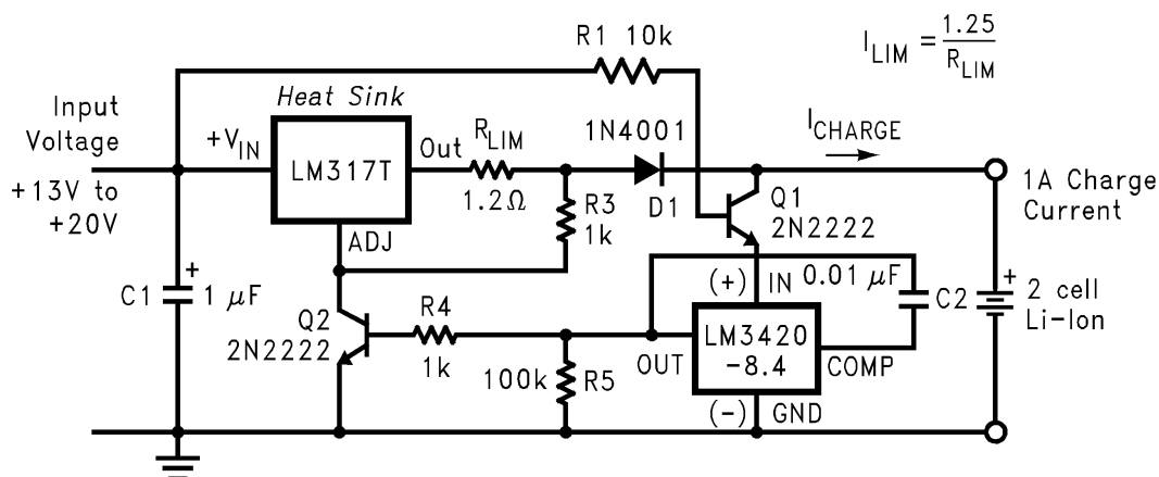
Simplified Schematic
