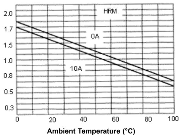
Operating Range Nominal Voltage Multiplying Factor
