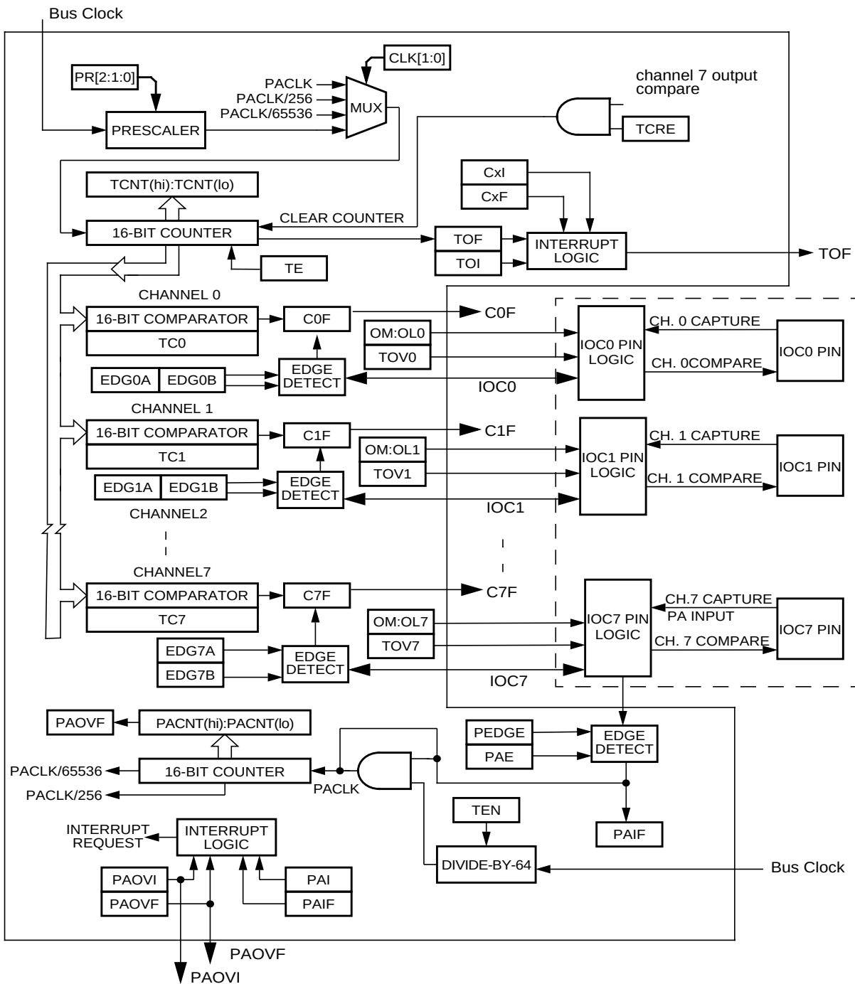
Figure 14-30. Detailed Timer Block Diagram
