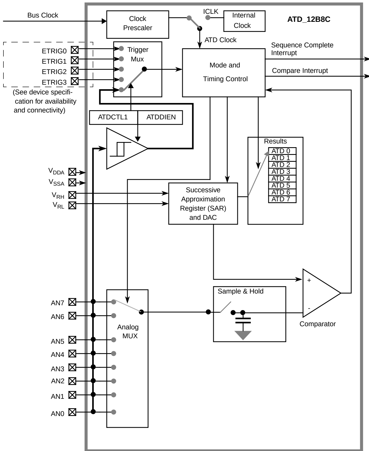
Figure 8-1. ADC12B8C Block Diagram
