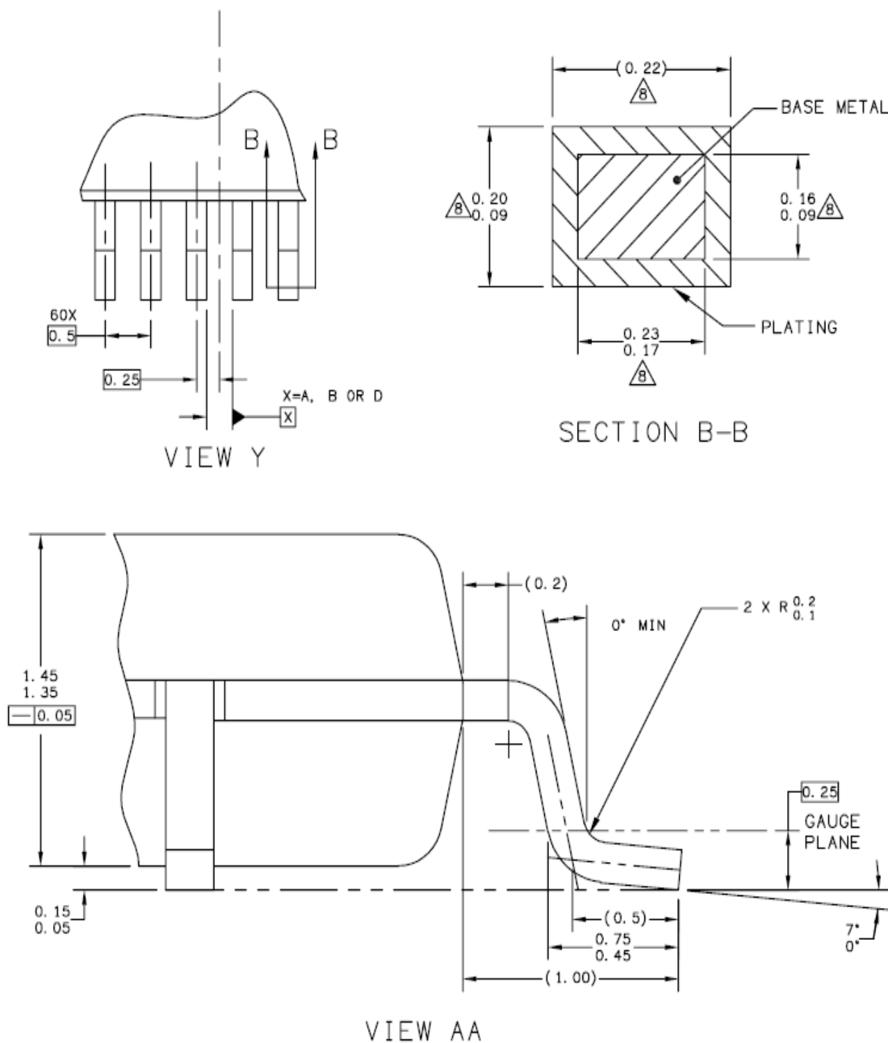
Figure C-5. 64-pin LQFP (case no. 840F) - page 2
