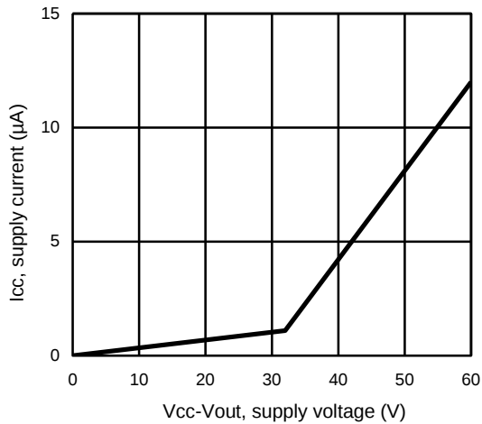
Figure 5 – Icc off (µA) Vs Vcc-Vout (V)
