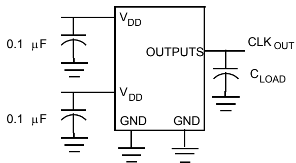
Figure 3. Test Circuit # 1
