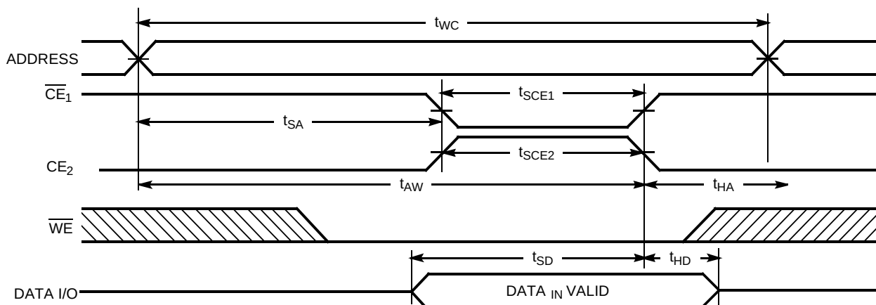
Write Cycle No. 2 ( \overline{CE} Controlled) [13,14,15]
