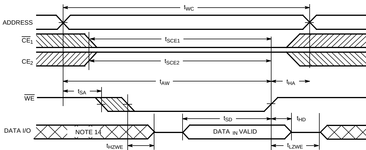
Write Cycle No. 3 ( \overline{WE} Controlled, \overline{OE} LOW) [13,14,15,16]
