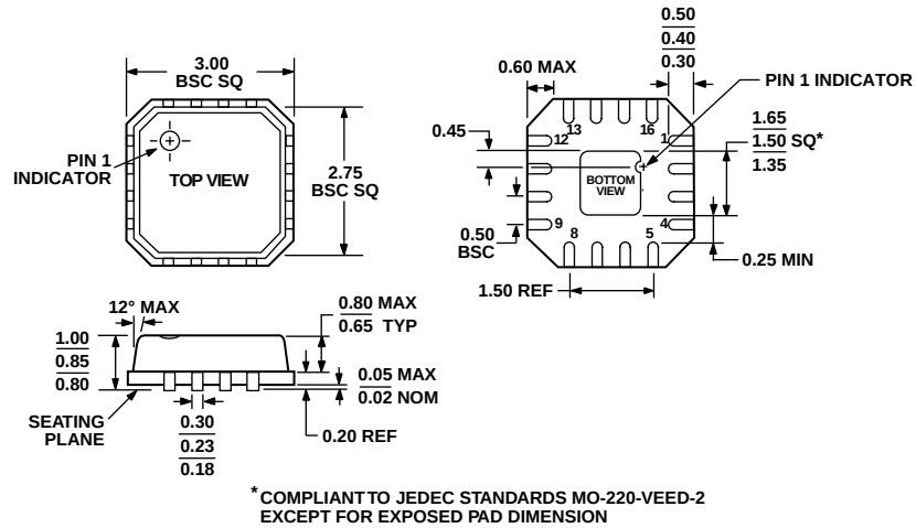
Figure 10. 16-Lead Lead Frame Chip Scale Package [LFCSP] 3 mm × 3 mm Body (CP-16-3) Dimensions shown in millimeters
