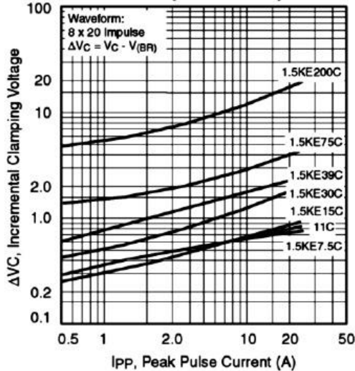
Fig. 7 – Incremental Clamping Voltage Curve (Bidirectional)
