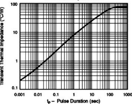
Fig. 13 – Typical Transient Thermal Impedance
