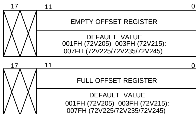
Figure 2. Writing to Offset Registers
